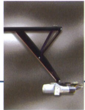
Stabilization jack with mini-hydraulic actuation.
