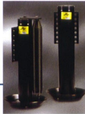
Hydraulic and electric leveling jacks.
